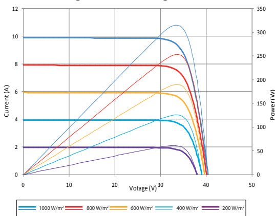
Current-Voltage & Power-Voltage Curve (315S-20)
